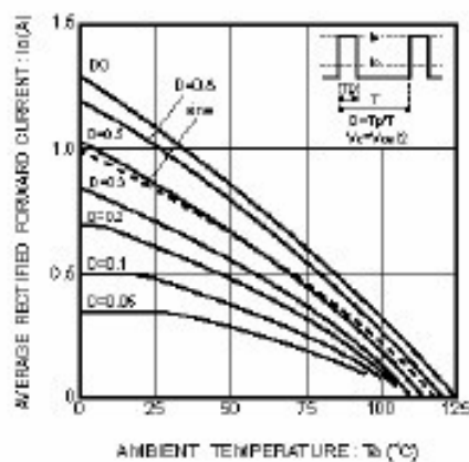
Fig.5 Derating curve ( I_o - T_a )
