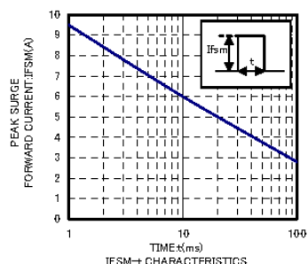
IFSM-t CHARACTERISTICS
