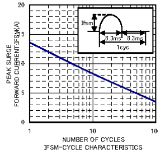
IFSM-CYCLE CHARACTERISTICS
