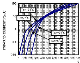
FORWARD VOLTAGE:VF(mV) VF-IF CHARACTERISTICS VF分布
