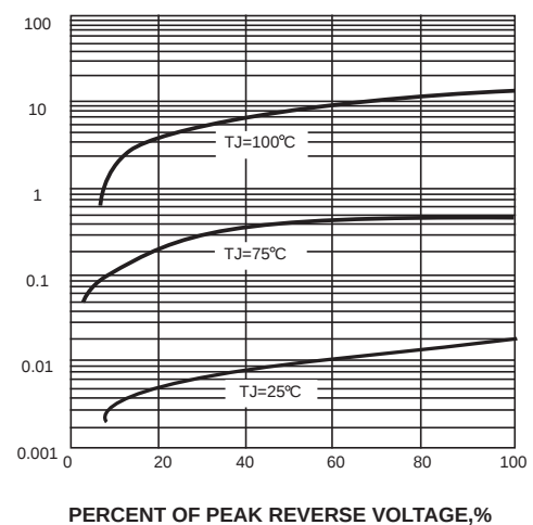
FIG. 4-TYPICAL REVERSE CHARACTERISTICS
