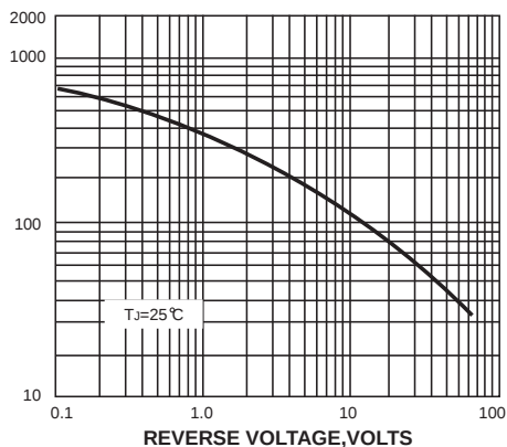
FIG. 5-TYPICAL JUNCTION CAPACITANCE
