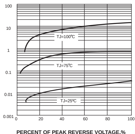
FIG. 4-TYPICAL REVERSE CHARACTERISTICS
